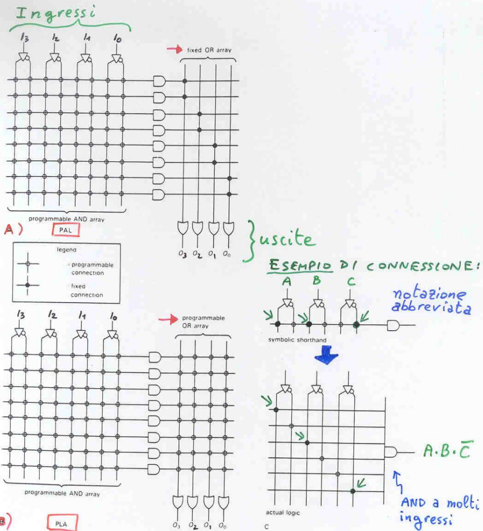
Figure 8.44. Programmable logic. A. PAL = PROGRAMMABLE ARRAY LOGIC B. PLA = PROGRAMMABLE LOGIC ARRAY C. Detail of programmable connections to many-input AND gate; the circles are fusible links or other programmable connections.
