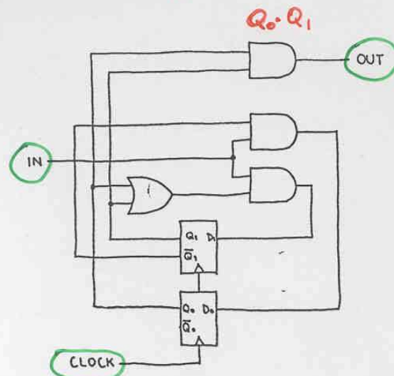
Figure X16.6: 011 detector: full circuit (conventional state machine design)
