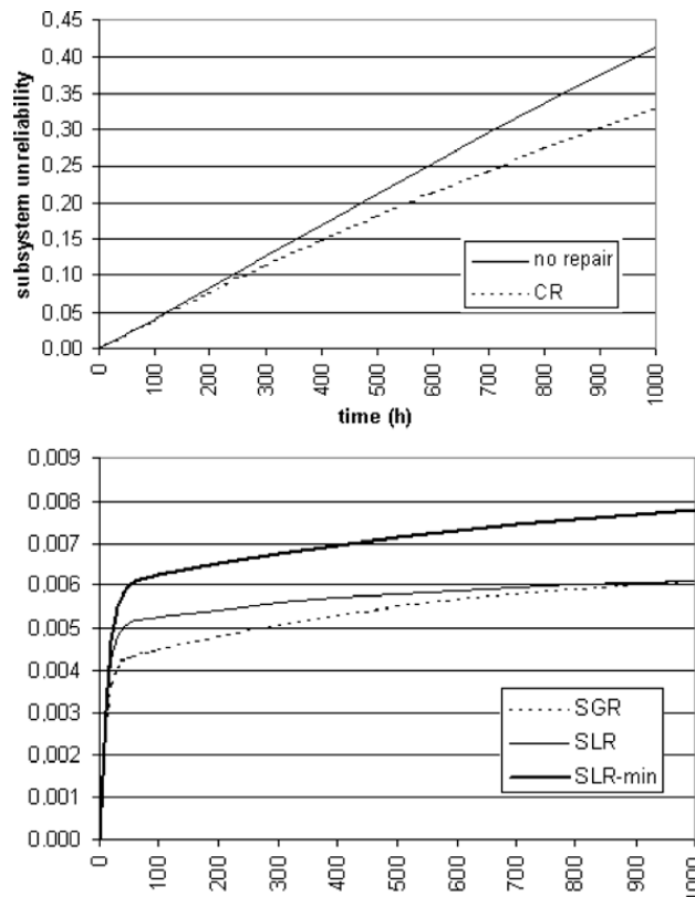
Fig. 8. The subsystem failure probability according to different repair policies.
