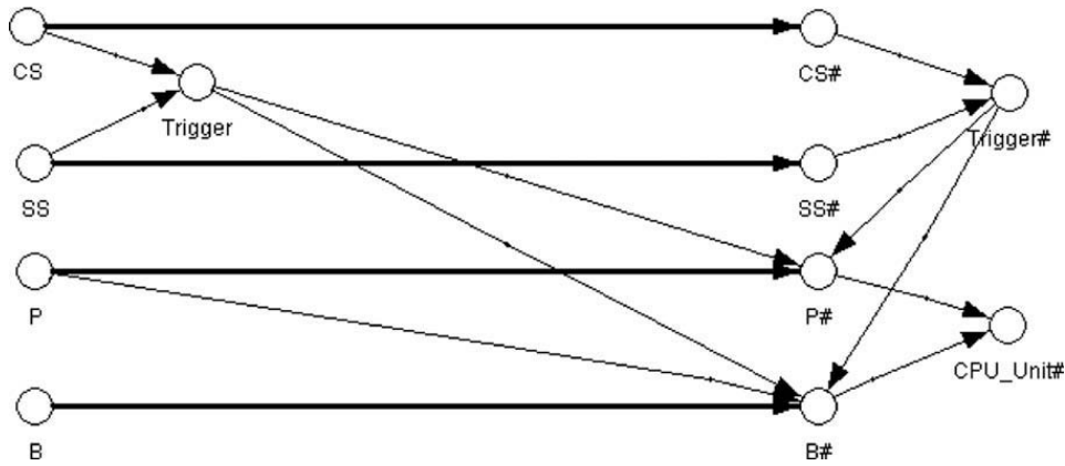
Fig. 5. A DBN for the CPU Unit subsystem with one-shot PDEP.
