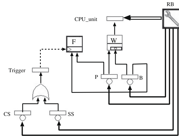
Fig. 3. A repair box (RB) modeling the repair of a subsystem, in case of Subsystem Global Repair (SGR) policy, Subsystem Local Repair (SLR) policy, or SLR-min policy.
