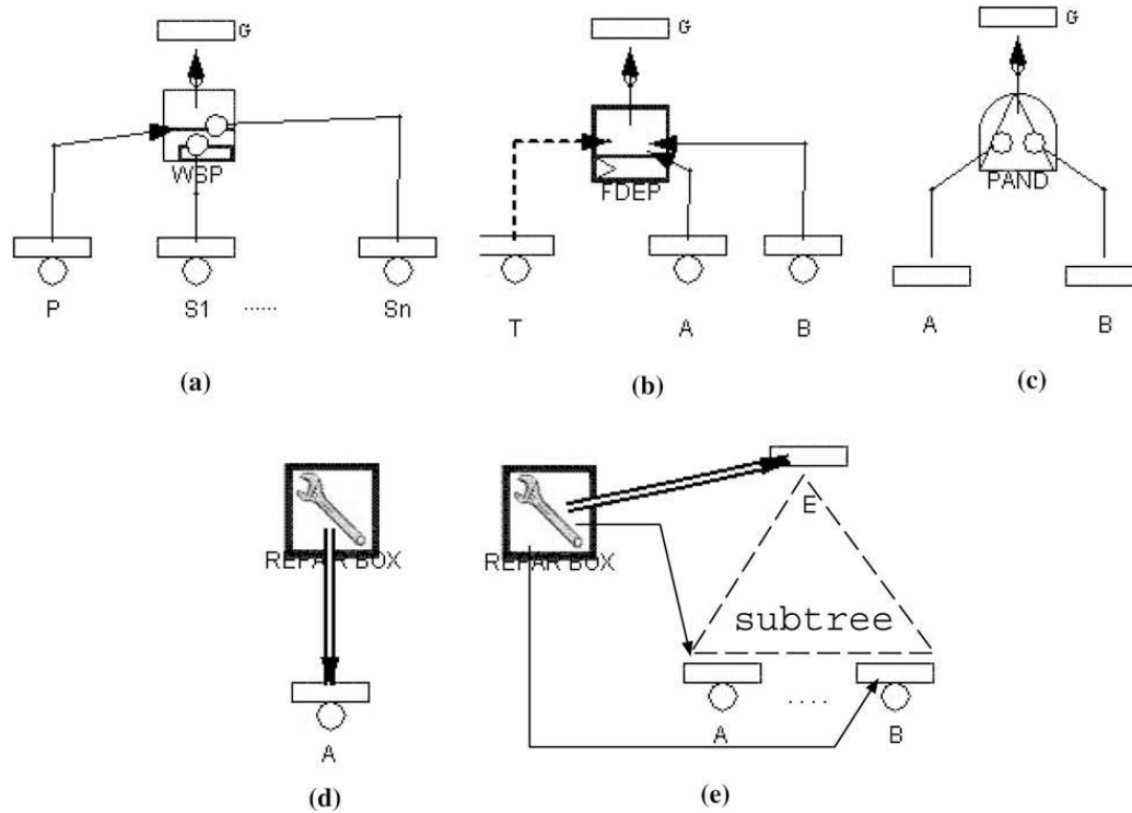
Fig. 1. Dynamic gates in a DFT.
