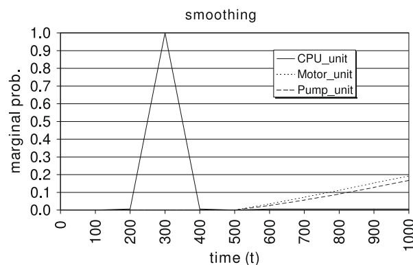
Fig. 12. The marginal probabilities in case of smoothing. Each curve indicates the failure probability of each subsystem.
