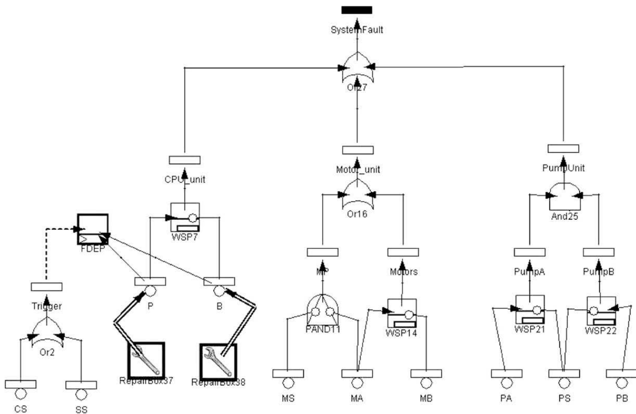
Fig. 9. The DFT model of CAS.
