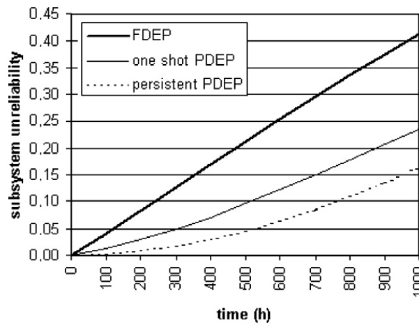
Fig. 6. The subsystem failure probability according to the type of functional dependency (using \pi_F = 0.5 in case of PDEP).
