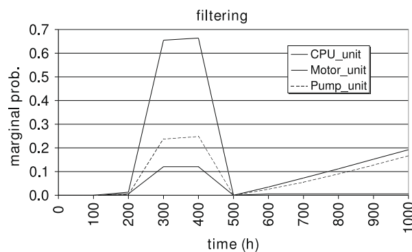
Fig. 11. The marginal probabilities in case of filtering. Each curve indicates the failure probability of each subsystem.
