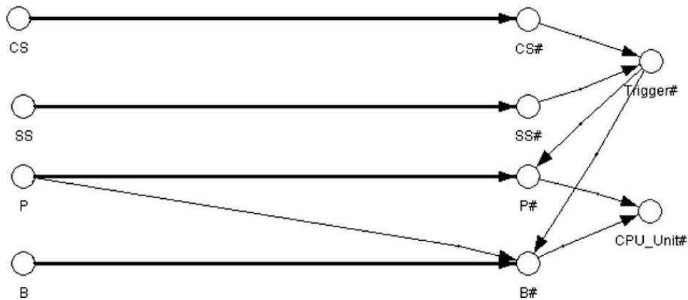
Fig. 4. A DBN for the CPU Unit subsystem.
